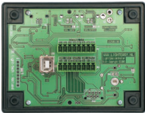
Rear side of Light-Easy
